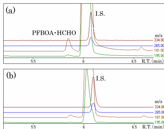
図 2 市販ビールにおける典型的なSIMクロマトグラム (a) Formaldehyde was detected at a level of 0.002 \mu\text{g/mL} . (b) Detectable level of formaldehyde was not detected.
